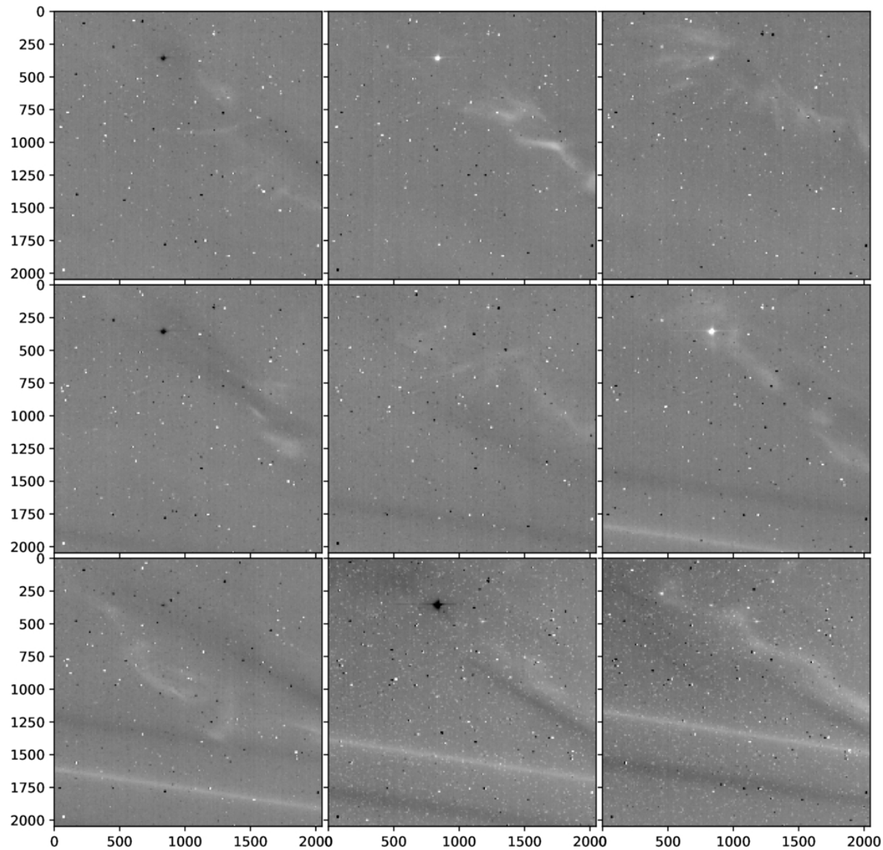
Figure 8. from Mike Alexandersen et al 2026 Planet. Sci. J. 7 doi:10.3847/PSJ/ae8a4d https://dx.doi.org/10.3847/PSJ/ae8a4d © 2026. The Author(s). Published by the American Astronomical Society.
