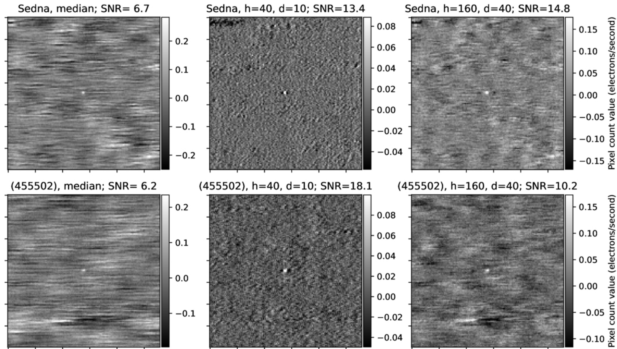
Figure 7. from Mike Alexandersen et al 2026 Planet. Sci. J. 7 doi:10.3847/PSJ/ae8a4d https://dx.doi.org/10.3847/PSJ/ae8a4d © 2026. The Author(s). Published by the American Astronomical Society.
