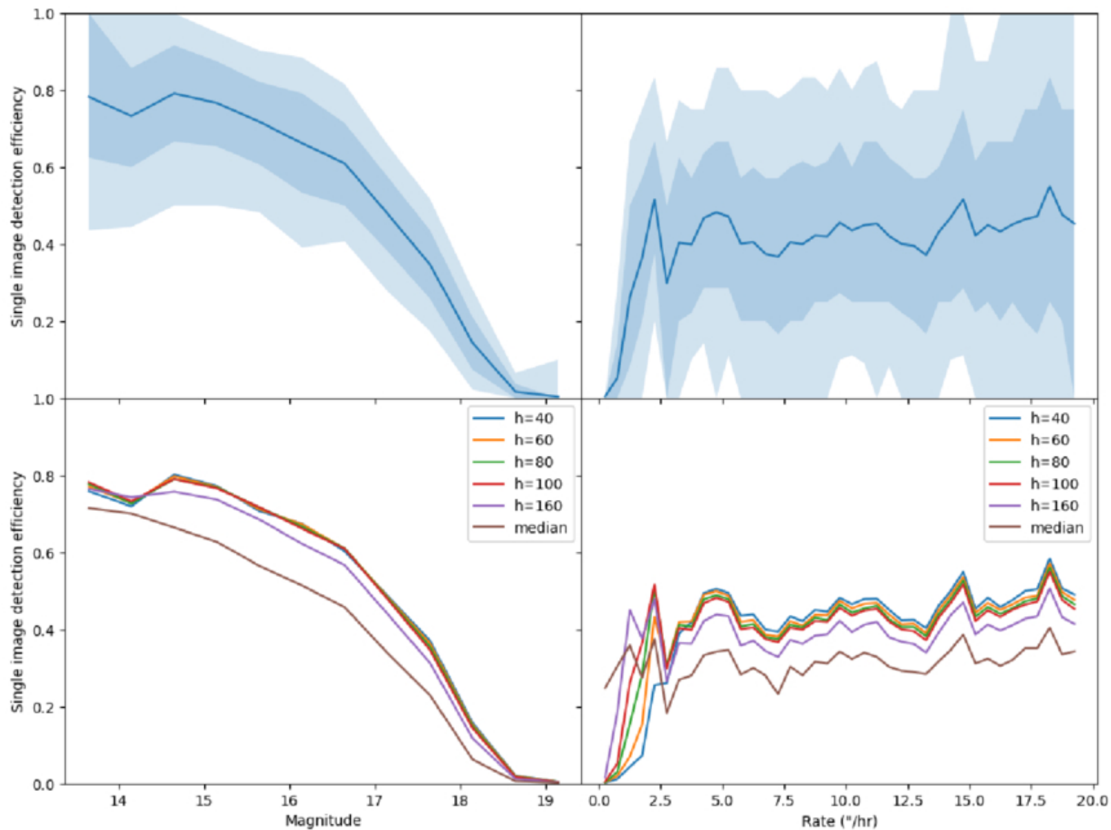
Figure 4. from Mike Alexandersen et al 2026 Planet. Sci. J. 7 doi:10.3847/PSJ/ae8a4d https://dx.doi.org/10.3847/PSJ/ae8a4d © 2026. The Author(s). Published by the American Astronomical Society.
