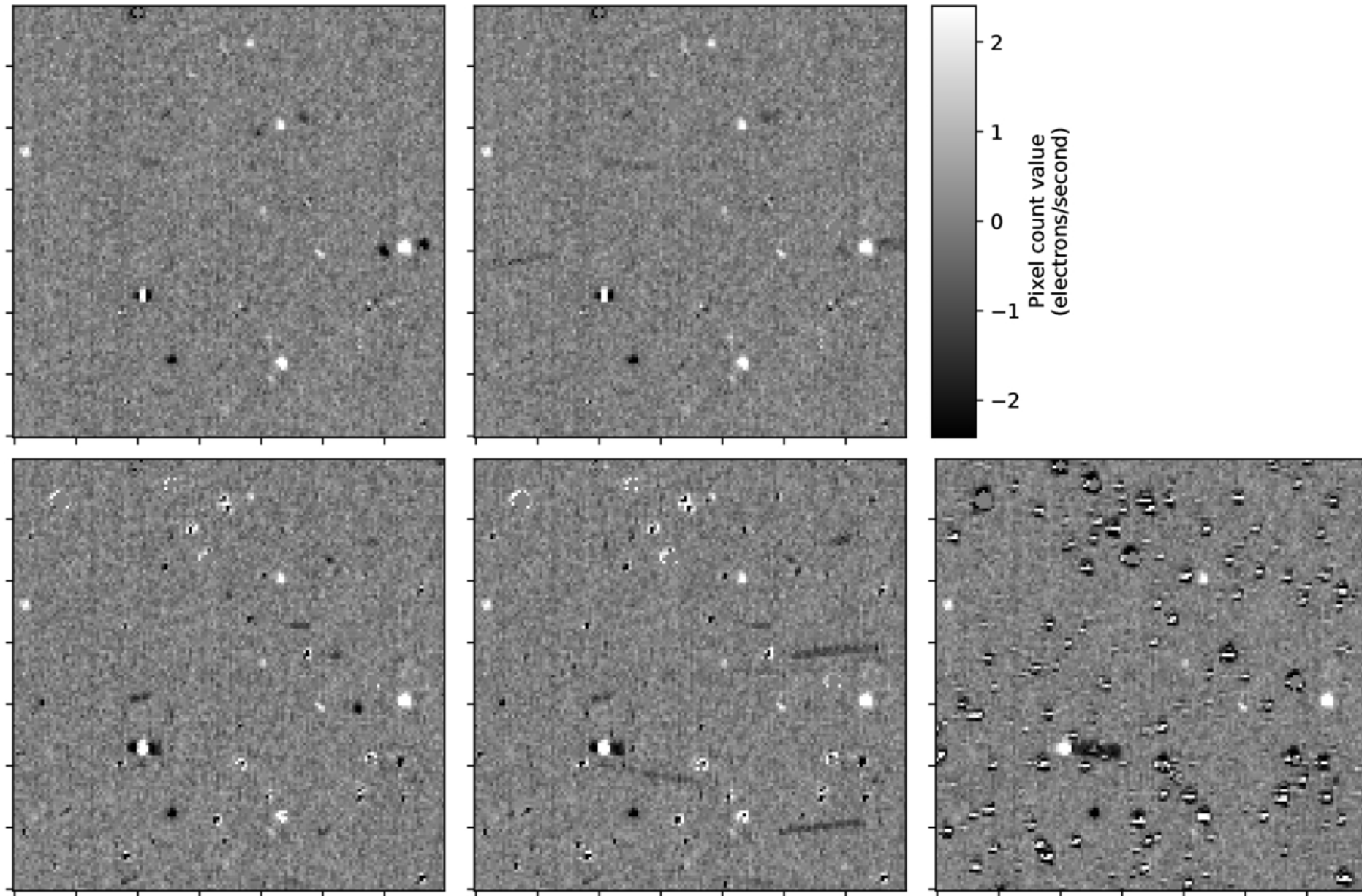
Figure 3. from Mike Alexandersen et al 2026 Planet. Sci. J. 7 doi:10.3847/PSJ/ae8a4d https://dx.doi.org/10.3847/PSJ/ae8a4d © 2026. The Author(s). Published by the American Astronomical Society.
