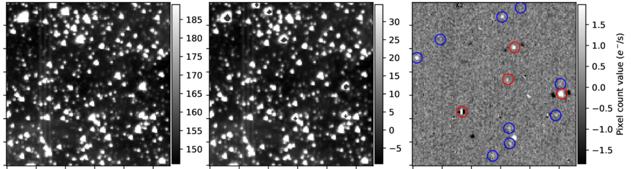
Figure 2. from Mike Alexandersen et al 2026 Planet. Sci. J. 7 doi:10.3847/PSJ/ae8a4d https://dx.doi.org/10.3847/PSJ/ae8a4d © 2026. The Author(s). Published by the American Astronomical Society.
