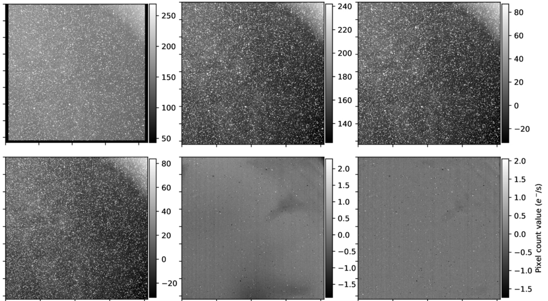
Figure 1. from Mike Alexandersen et al 2026 Planet. Sci. J. 7 doi:10.3847/PSJ/ae8a4d https://dx.doi.org/10.3847/PSJ/ae8a4d © 2026. The Author(s). Published by the American Astronomical Society.
