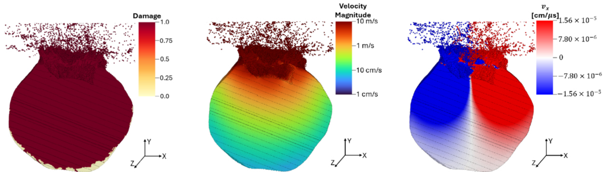
Figure 9. from Isaiah B. Santistevan et al 2026 Planet. Sci. J. 7 doi:10.3847/PSJ/ae8a49 https://dx.doi.org/10.3847/PSJ/ae8a49 © 2026. The Author(s). Published by the American Astronomical Society.
