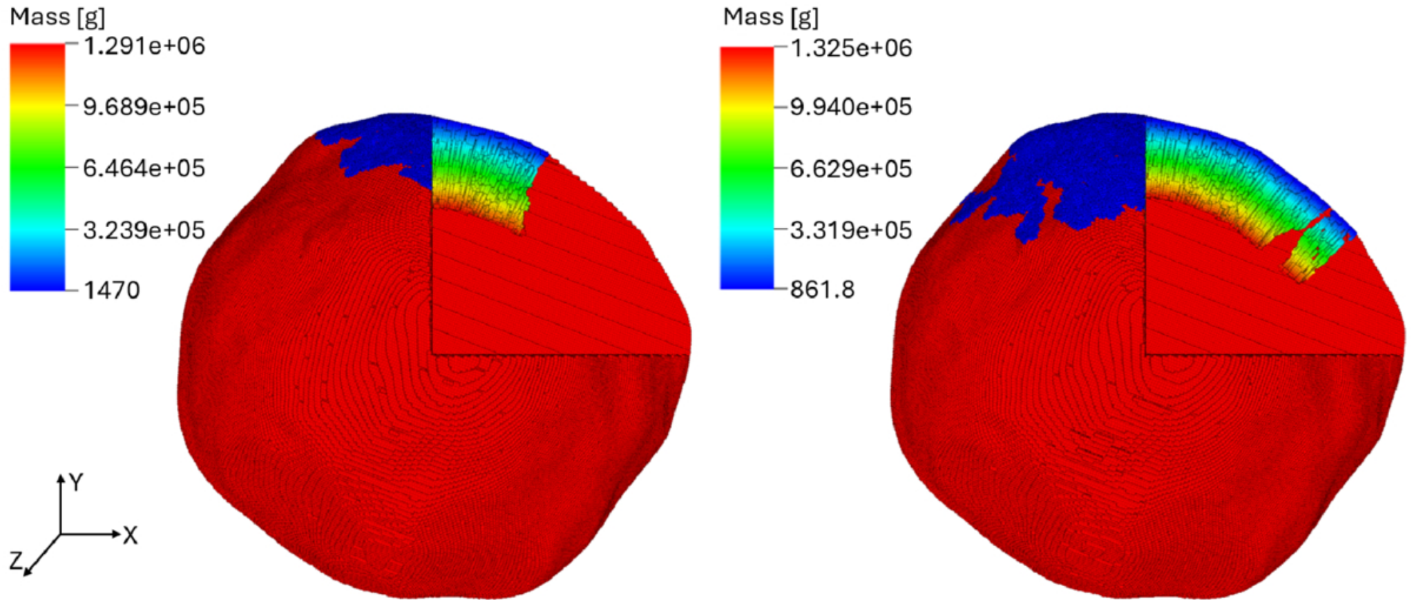
Figure 8. from Isaiah B. Santistevan et al 2026 Planet. Sci. J. 7 doi:10.3847/PSJ/ae8a49 https://dx.doi.org/10.3847/PSJ/ae8a49 © 2026. The Author(s). Published by the American Astronomical Society.
