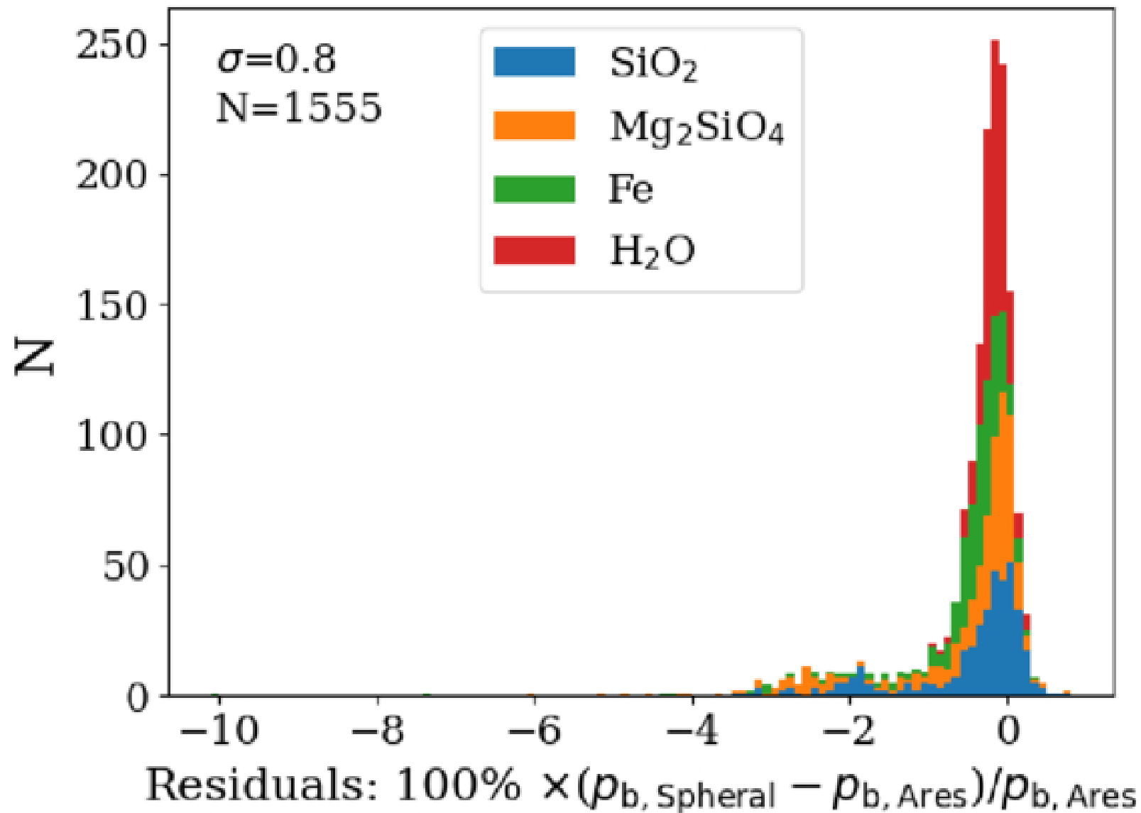
Figure 3. from Isaiah B. Santistevan et al 2026 Planet. Sci. J. 7 doi:10.3847/PSJ/ae8a49 https://dx.doi.org/10.3847/PSJ/ae8a49 © 2026. The Author(s). Published by the American Astronomical Society.
