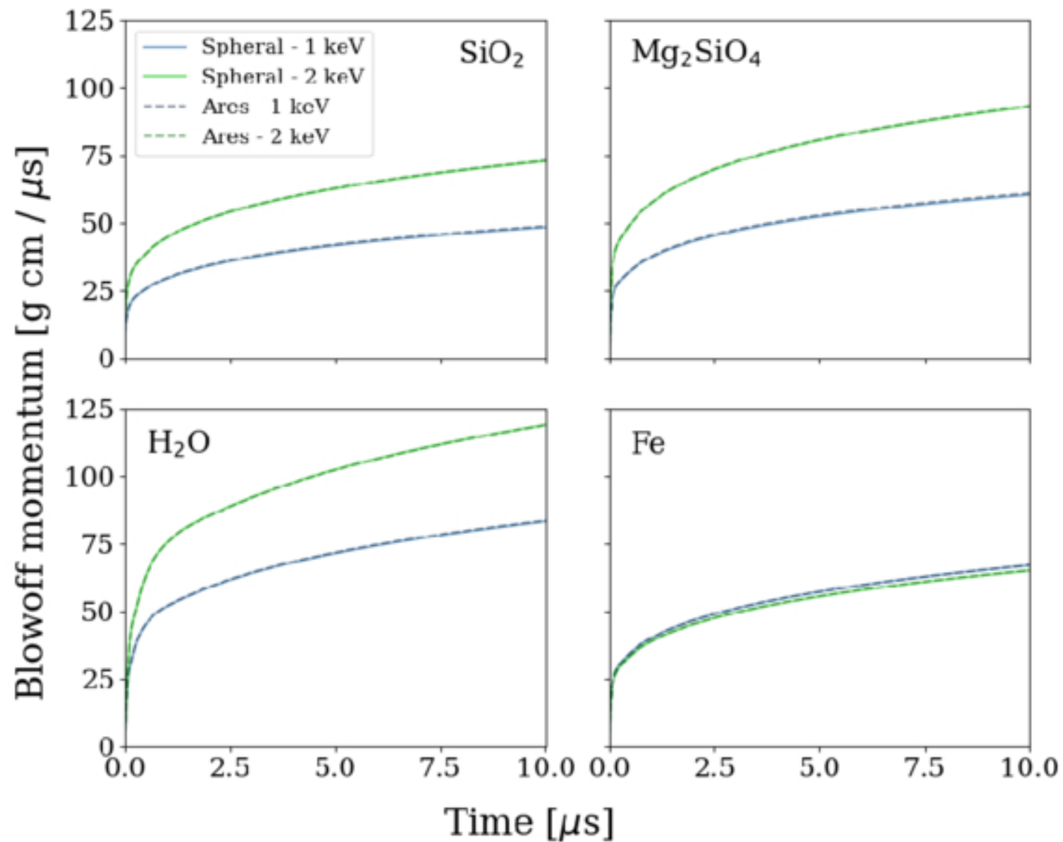
Figure 2. from Isaiah B. Santistevan et al 2026 Planet. Sci. J. 7 doi:10.3847/PSJ/ae8a49 https://dx.doi.org/10.3847/PSJ/ae8a49 © 2026. The Author(s). Published by the American Astronomical Society.
