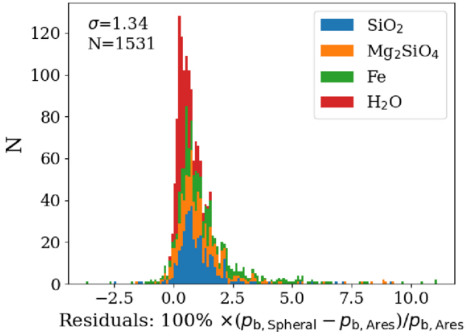
Figure C1. from Isaiah B. Santistevan et al 2026 Planet. Sci. J. 7 doi:10.3847/PSJ/ae8a49 https://dx.doi.org/10.3847/PSJ/ae8a49 © 2026. The Author(s). Published by the American Astronomical Society.
