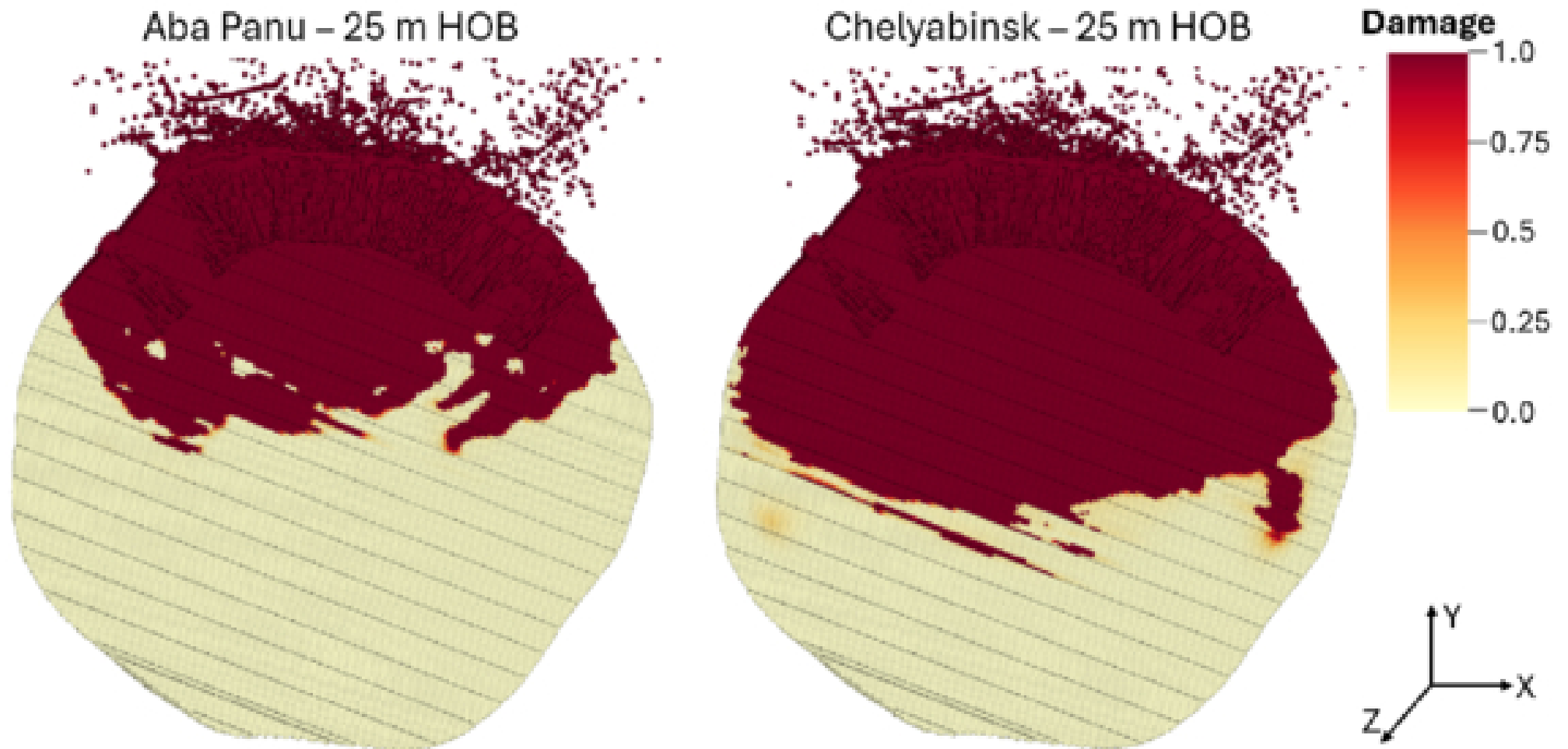
Figure 11. from Isaiah B. Santistevan et al 2026 Planet. Sci. J. 7 doi:10.3847/PSJ/ae8a49 https://dx.doi.org/10.3847/PSJ/ae8a49 © 2026. The Author(s). Published by the American Astronomical Society.
