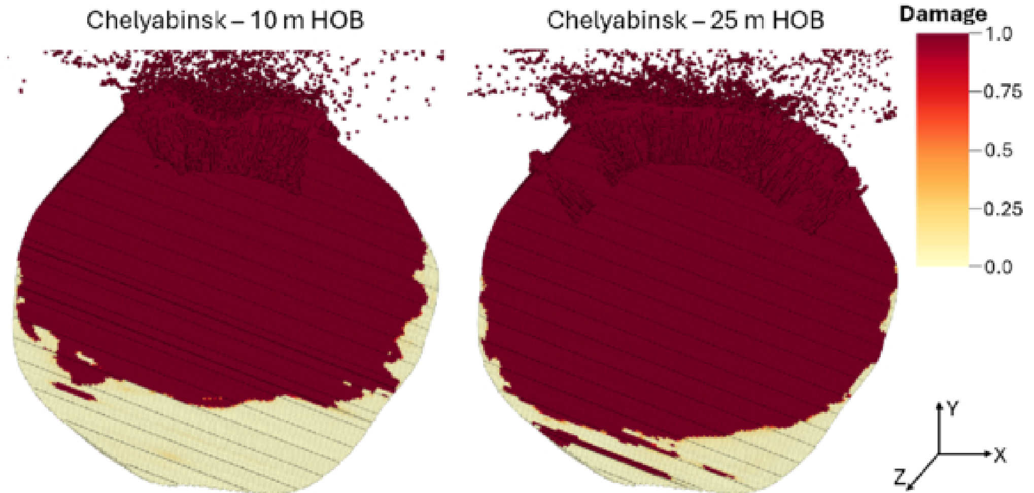
Figure 10. from Isaiah B. Santistevan et al 2026 Planet. Sci. J. 7 doi:10.3847/PSJ/ae8a49 https://dx.doi.org/10.3847/PSJ/ae8a49 © 2026. The Author(s). Published by the American Astronomical Society.
