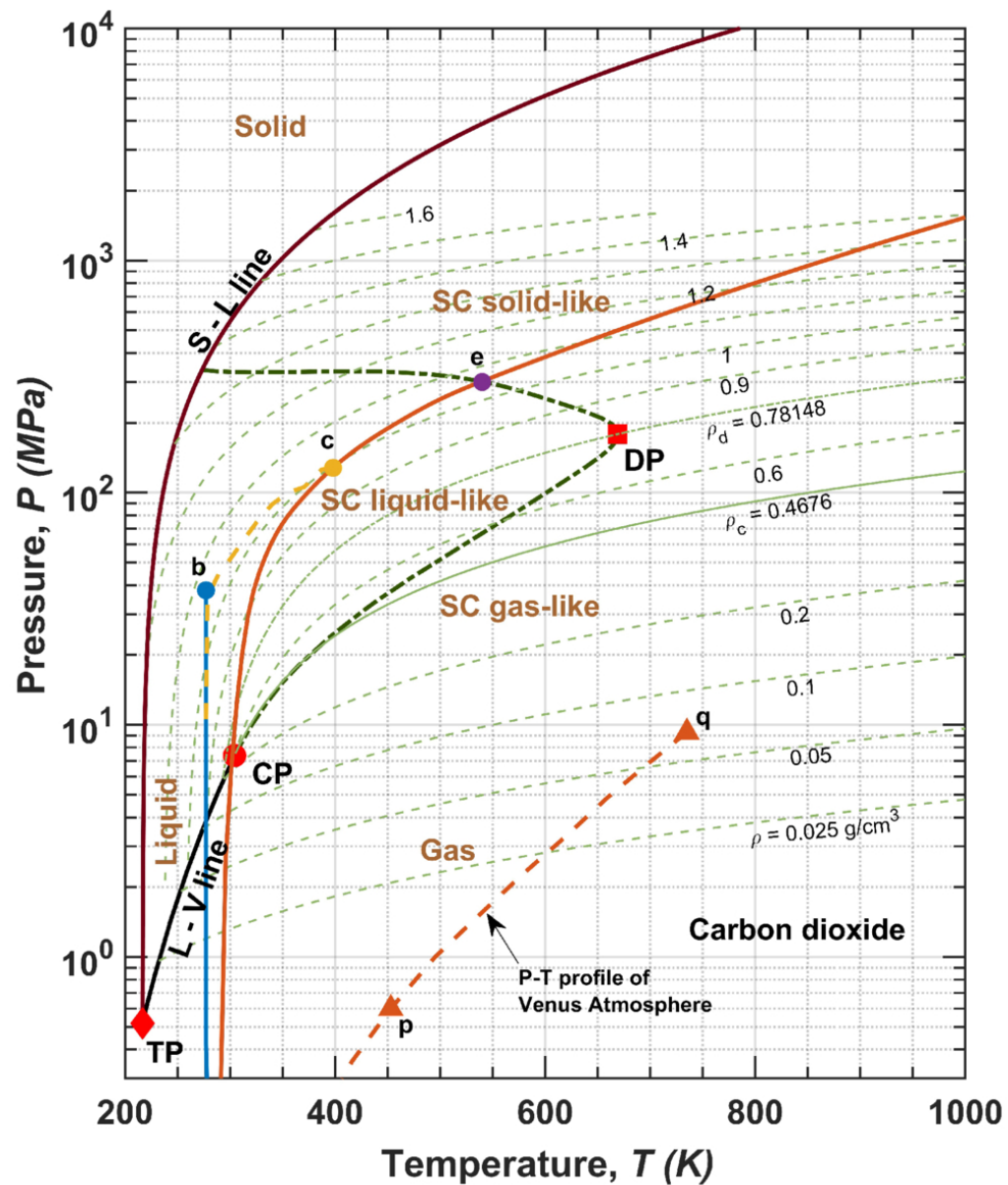
Figure 6. from Raad Shahmat Haque et al 2026 Planet. Sci. J. 7 doi:10.3847/PSJ/ae89b3 https://dx.doi.org/10.3847/PSJ/ae89b3 © 2026. The Author(s). Published by the American Astronomical Society.
