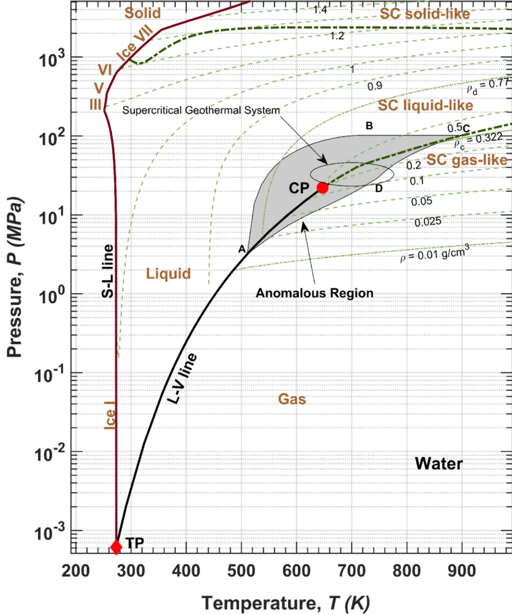
Figure 4. from Raad Shahmat Haque et al 2026 Planet. Sci. J. 7 doi:10.3847/PSJ/ae89b3 https://dx.doi.org/10.3847/PSJ/ae89b3 © 2026. The Author(s). Published by the American Astronomical Society.
