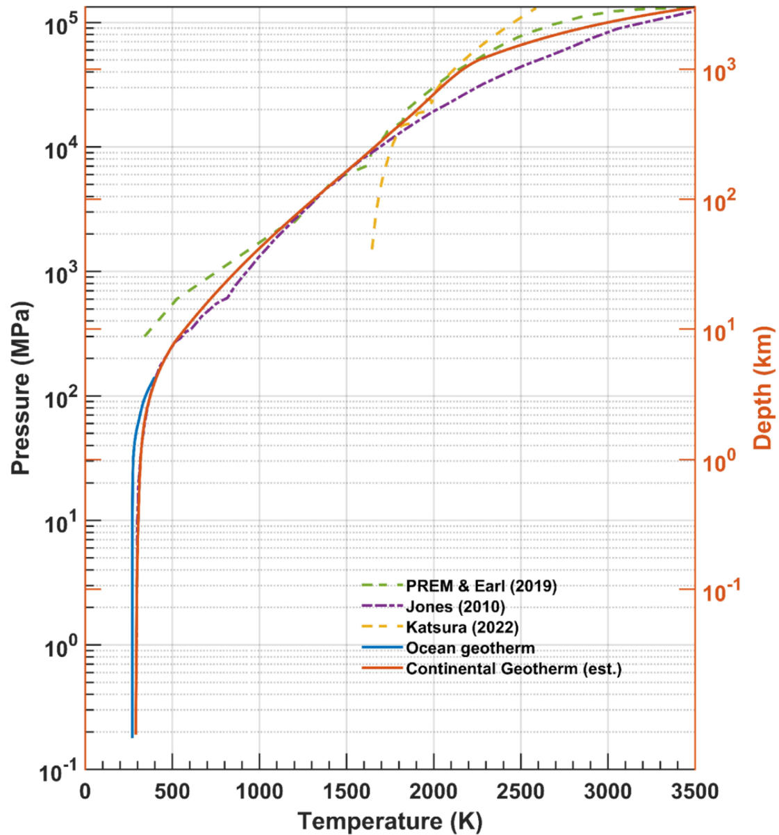
Figure 2. from Raad Shahmat Haque et al 2026 Planet. Sci. J. 7 doi:10.3847/PSJ/ae89b3 https://dx.doi.org/10.3847/PSJ/ae89b3 © 2026. The Author(s). Published by the American Astronomical Society.
