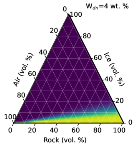
Figure 8. from Samuel W. Courville et al 2026 Planet. Sci. J. 7 doi:10.3847/PSJ/ae8904 https://dx.doi.org/10.3847/PSJ/ae8904 © 2026. The Author(s). Published by the American Astronomical Society.
