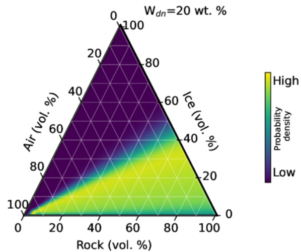
Figure 8. from Samuel W. Courville et al 2026 Planet. Sci. J. 7 doi:10.3847/PSJ/ae8904 https://dx.doi.org/10.3847/PSJ/ae8904 © 2026. The Author(s). Published by the American Astronomical Society.
