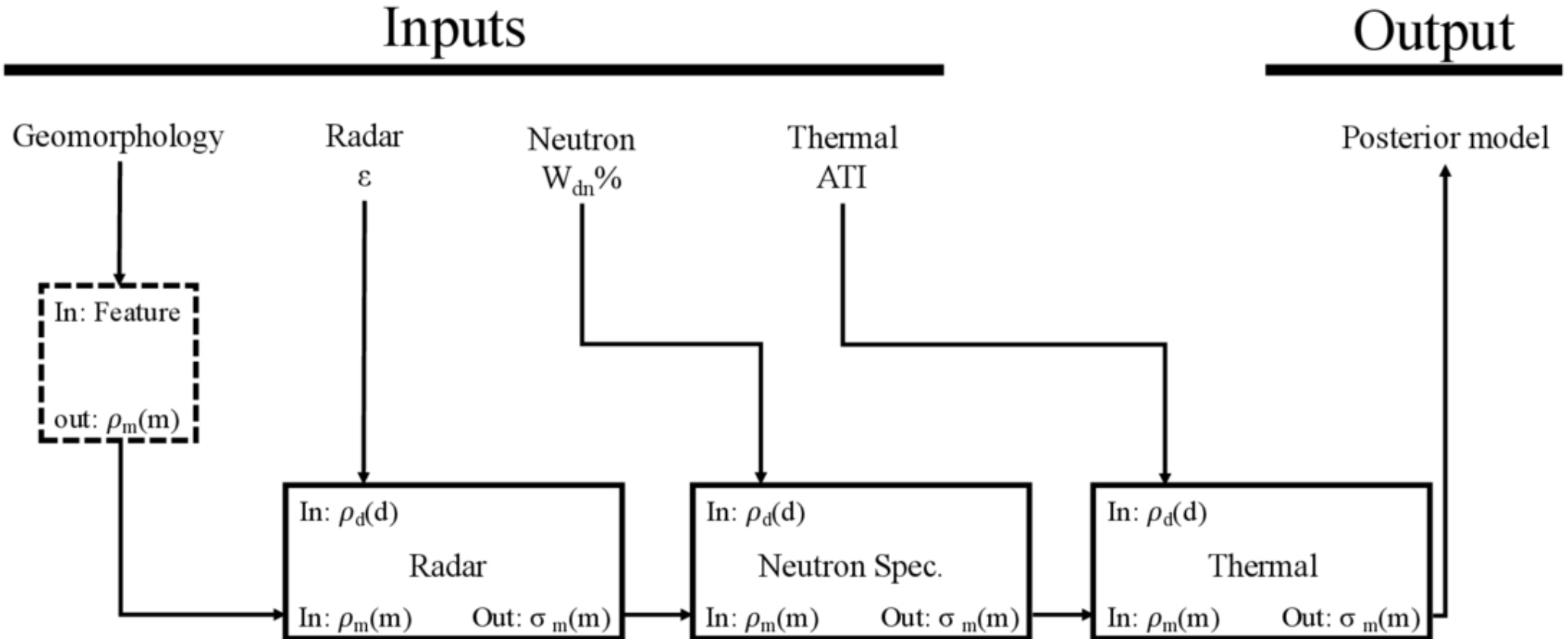
Figure 3. from Samuel W. Courville et al 2026 Planet. Sci. J. 7 doi:10.3847/PSJ/ae8904 https://dx.doi.org/10.3847/PSJ/ae8904 © 2026. The Author(s). Published by the American Astronomical Society.
