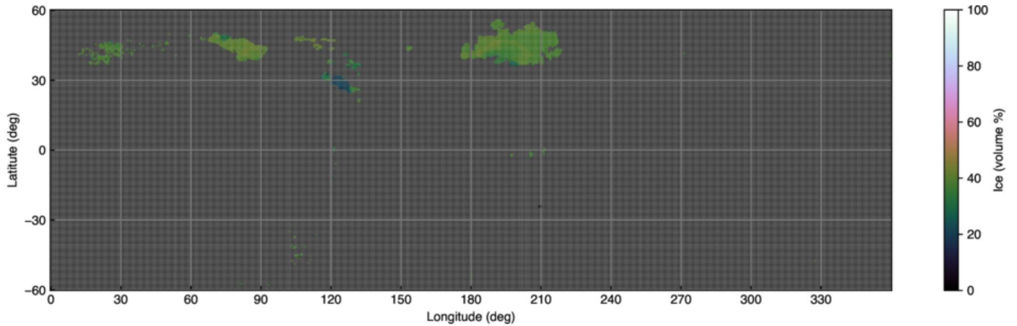
Figure 23. from Samuel W. Courville et al 2026 Planet. Sci. J. 7 doi:10.3847/PSJ/ae8904 https://dx.doi.org/10.3847/PSJ/ae8904 © 2026. The Author(s). Published by the American Astronomical Society.
