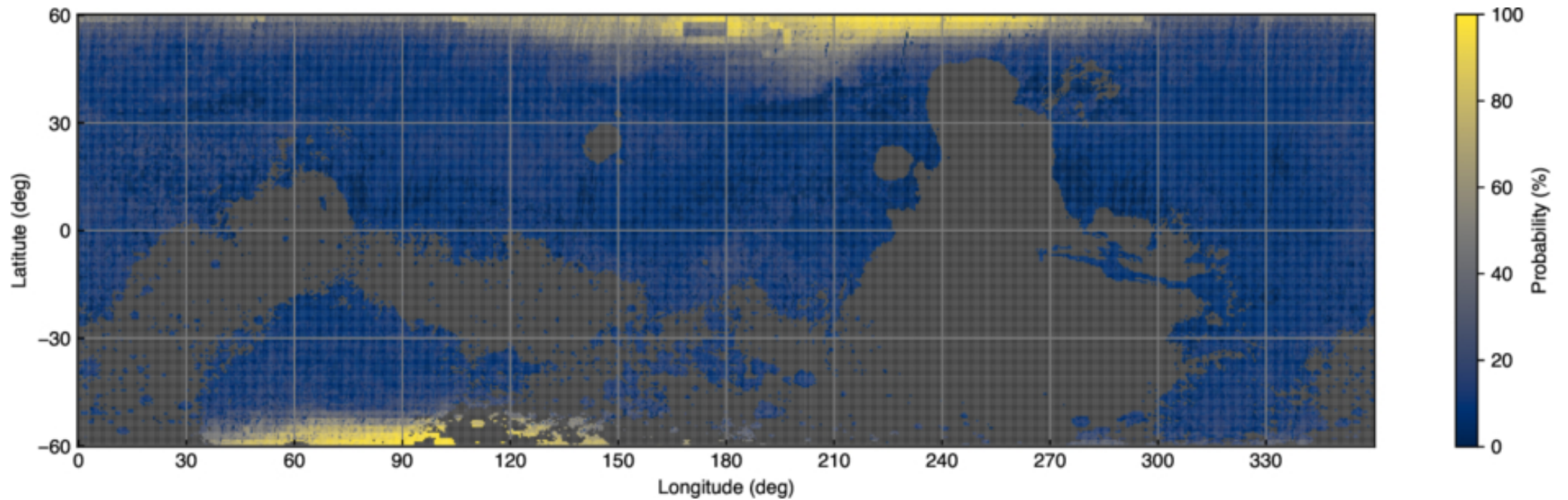
Figure 22. from Samuel W. Courville et al 2026 Planet. Sci. J. 7 doi:10.3847/PSJ/ae8904 https://dx.doi.org/10.3847/PSJ/ae8904 © 2026. The Author(s). Published by the American Astronomical Society.
