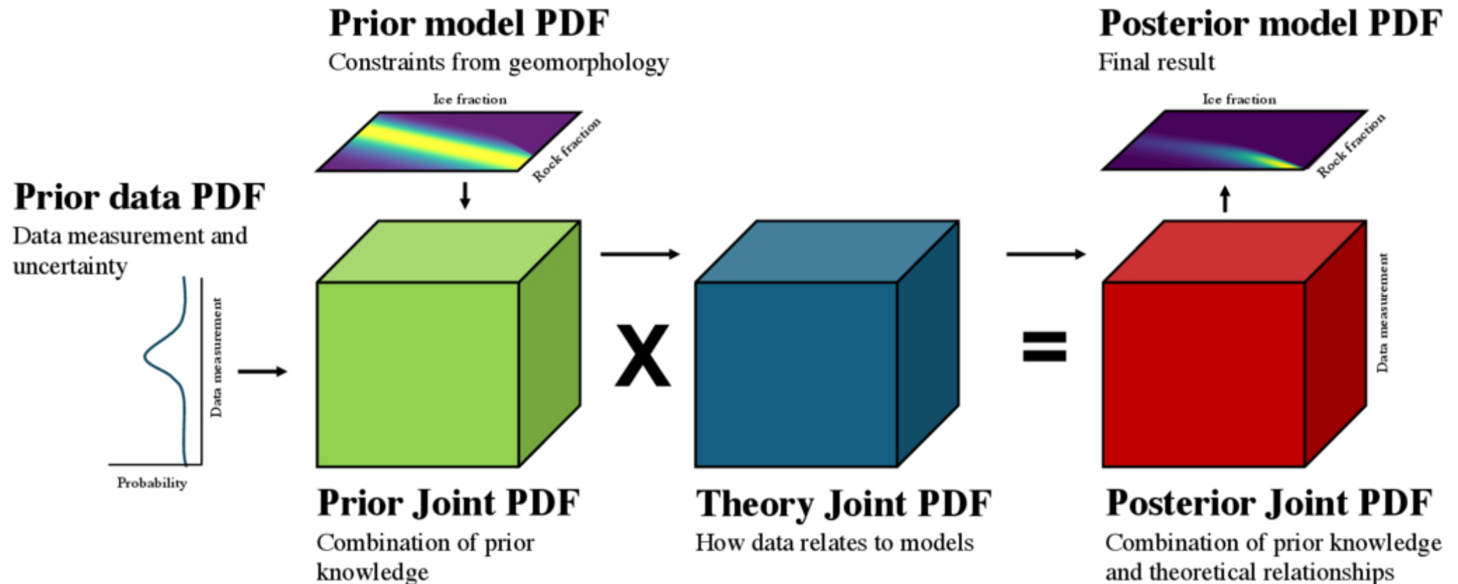
Figure 2. from Samuel W. Courville et al 2026 Planet. Sci. J. 7 doi:10.3847/PSJ/ae8904 https://dx.doi.org/10.3847/PSJ/ae8904 © 2026. The Author(s). Published by the American Astronomical Society.
