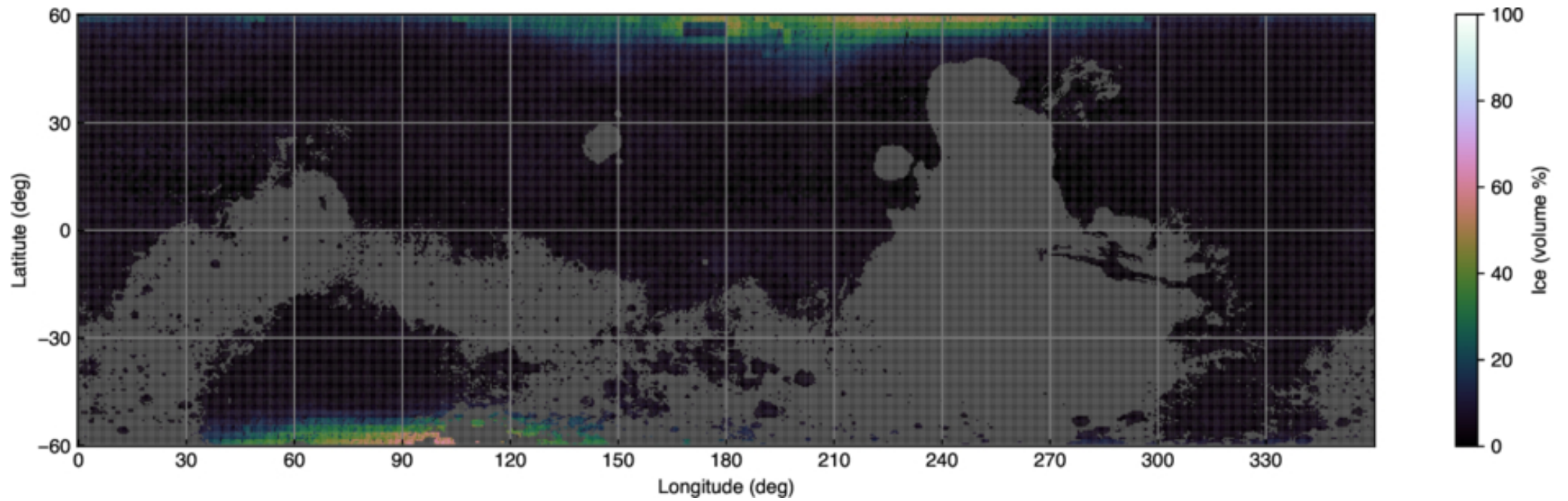
Figure 19. from Samuel W. Courville et al 2026 Planet. Sci. J. 7 doi:10.3847/PSJ/ae8904 https://dx.doi.org/10.3847/PSJ/ae8904 © 2026. The Author(s). Published by the American Astronomical Society.
