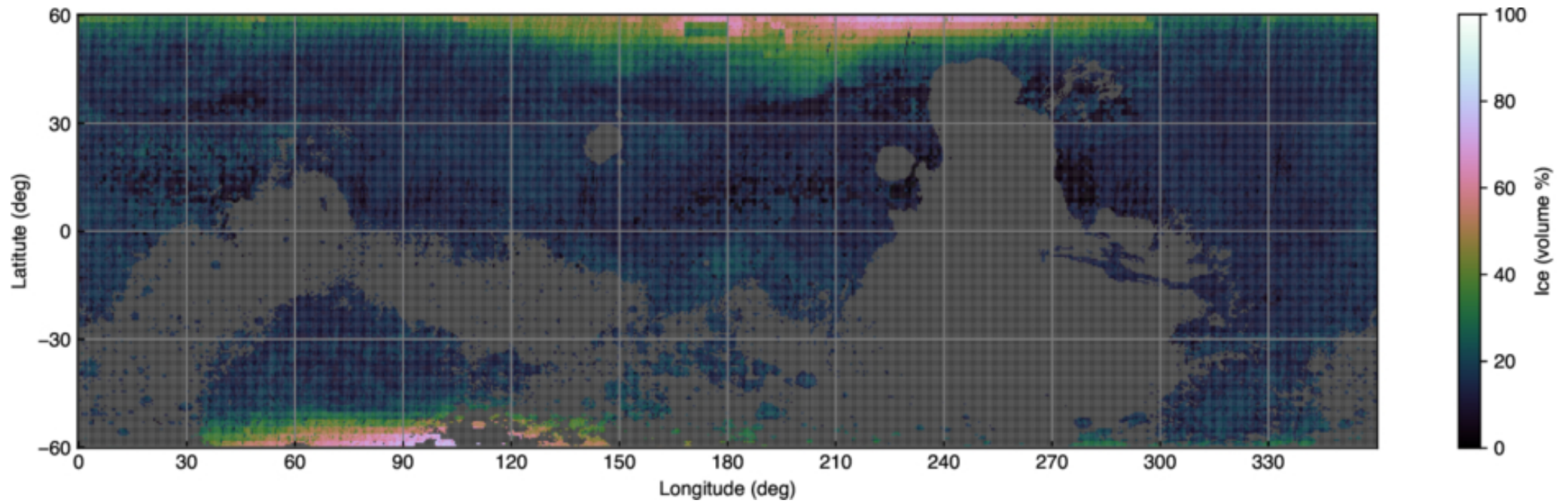
Figure 18. from Samuel W. Courville et al 2026 Planet. Sci. J. 7 doi:10.3847/PSJ/ae8904 https://dx.doi.org/10.3847/PSJ/ae8904 © 2026. The Author(s). Published by the American Astronomical Society.
