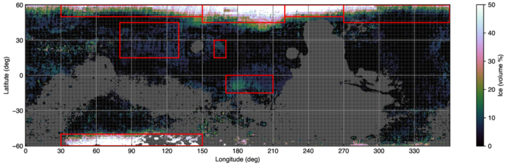
Figure 17. from Samuel W. Courville et al 2026 Planet. Sci. J. 7 doi:10.3847/PSJ/ae8904 https://dx.doi.org/10.3847/PSJ/ae8904 © 2026. The Author(s). Published by the American Astronomical Society.
