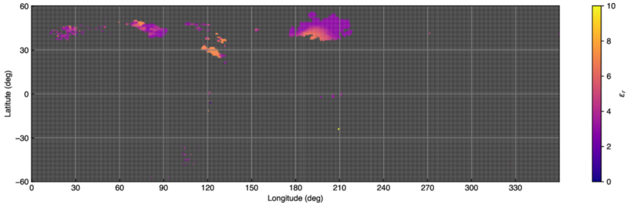
Figure 14. from Samuel W. Courville et al 2026 Planet. Sci. J. 7 doi:10.3847/PSJ/ae8904 https://dx.doi.org/10.3847/PSJ/ae8904 © 2026. The Author(s). Published by the American Astronomical Society.
