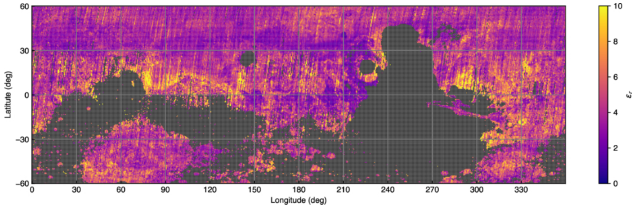
Figure 13. from Samuel W. Courville et al 2026 Planet. Sci. J. 7 doi:10.3847/PSJ/ae8904 https://dx.doi.org/10.3847/PSJ/ae8904 © 2026. The Author(s). Published by the American Astronomical Society.
