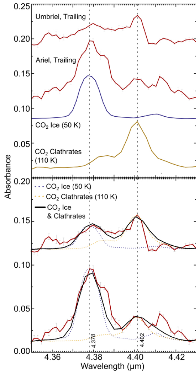
Figure 8. from Richard J. Cartwright et al 2026 Planet. Sci. J. 7 doi:10.3847/PSJ/ae8818 https://dx.doi.org/10.3847/PSJ/ae8818 © 2026. The Author(s). Published by the American Astronomical Society.
