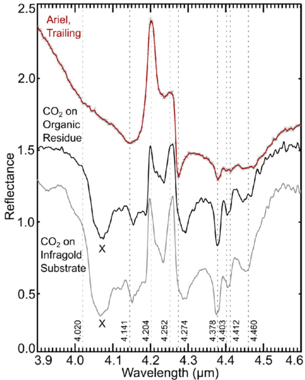
Figure 6. from Richard J. Cartwright et al 2026 Planet. Sci. J. 7 doi:10.3847/PSJ/ae8818 https://dx.doi.org/10.3847/PSJ/ae8818 © 2026. The Author(s). Published by the American Astronomical Society.
