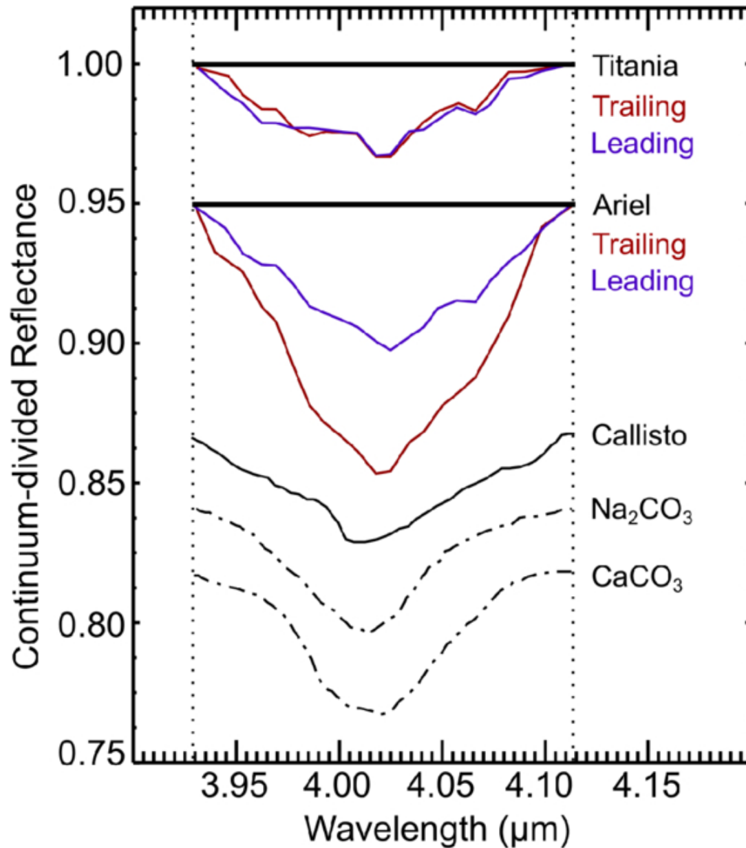
Figure 10. from Richard J. Cartwright et al 2026 Planet. Sci. J. 7 doi:10.3847/PSJ/ae8818 https://dx.doi.org/10.3847/PSJ/ae8818 © 2026. The Author(s). Published by the American Astronomical Society.
