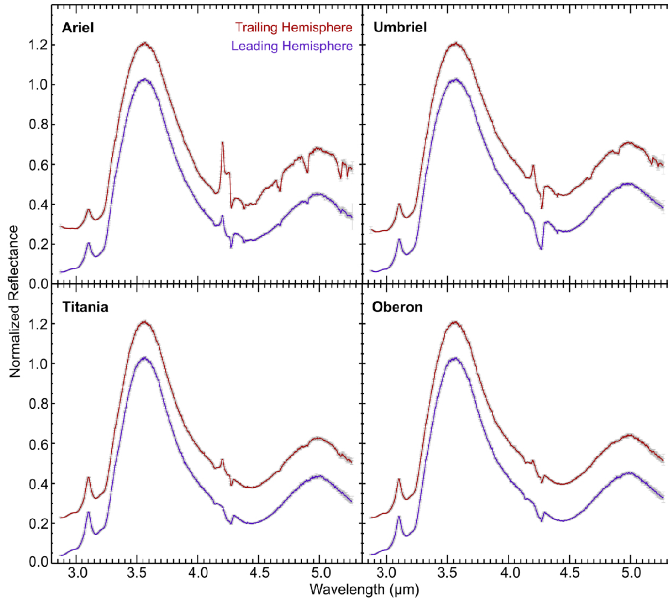
Figure 1. from Richard J. Cartwright et al 2026 Planet. Sci. J. 7 doi:10.3847/PSJ/ae8818 https://dx.doi.org/10.3847/PSJ/ae8818 © 2026. The Author(s). Published by the American Astronomical Society.
