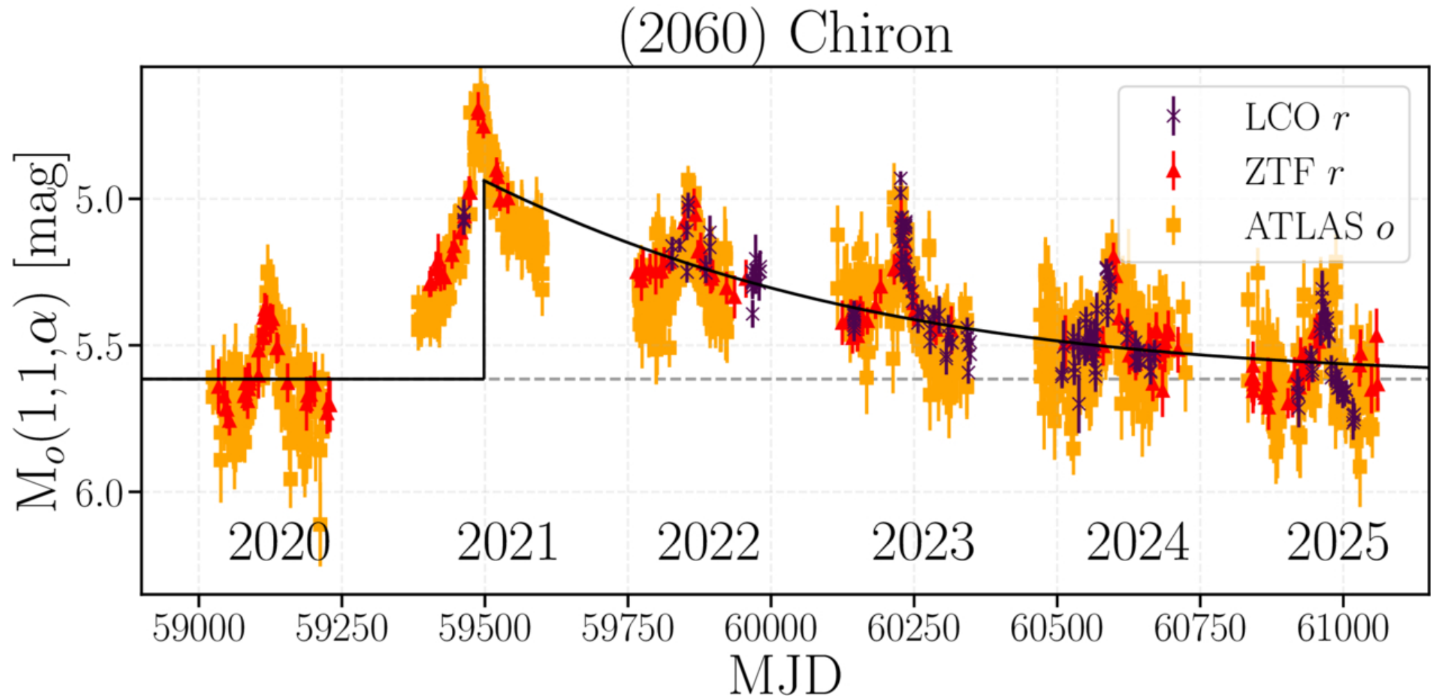
Figure 9. from Joseph Murtagh et al 2026 Planet. Sci. J. 7 doi:10.3847/PSJ/ae8790 https://dx.doi.org/10.3847/PSJ/ae8790 © 2026. The Author(s). Published by the American Astronomical Society.
