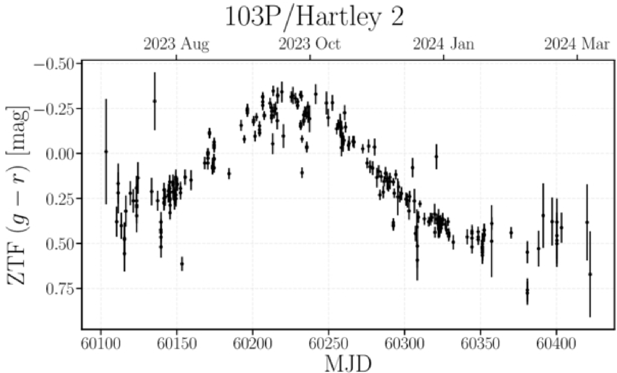
Figure 5. from Joseph Murtagh et al 2026 Planet. Sci. J. 7 doi:10.3847/PSJ/ae8790 https://dx.doi.org/10.3847/PSJ/ae8790 © 2026. The Author(s). Published by the American Astronomical Society.
