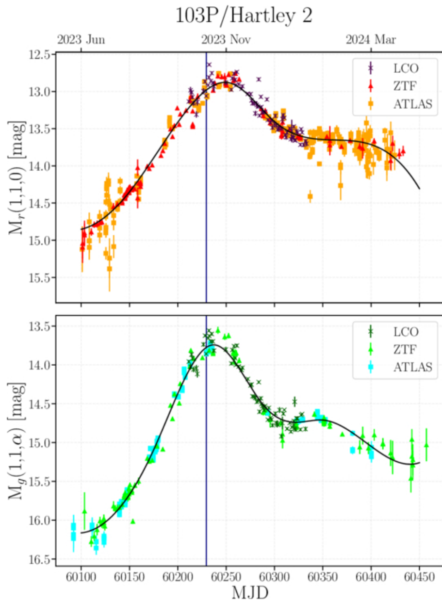
Figure 3. from Joseph Murtagh et al 2026 Planet. Sci. J. 7 doi:10.3847/PSJ/ae8790 https://dx.doi.org/10.3847/PSJ/ae8790 © 2026. The Author(s). Published by the American Astronomical Society.
