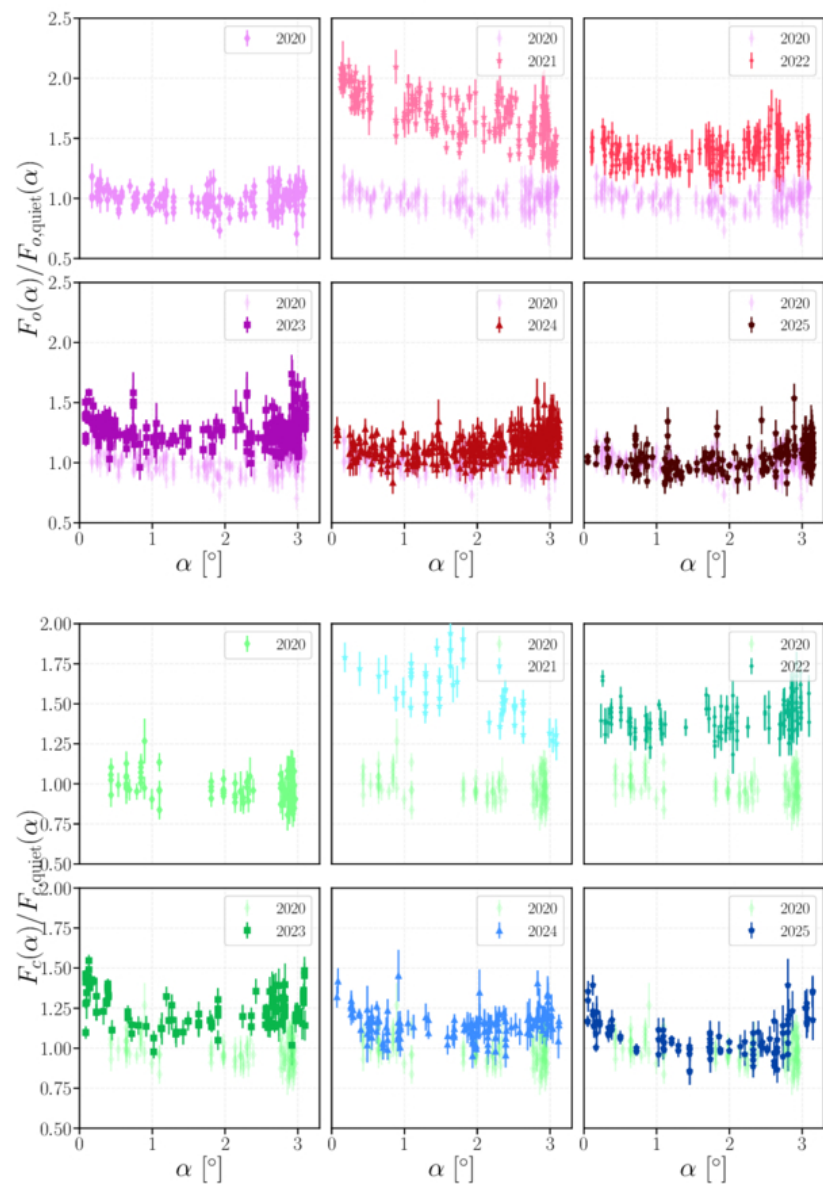
Figure 10. from Joseph Murtagh et al 2026 Planet. Sci. J. 7 doi:10.3847/PSJ/ae8790 https://dx.doi.org/10.3847/PSJ/ae8790 © 2026. The Author(s). Published by the American Astronomical Society.
