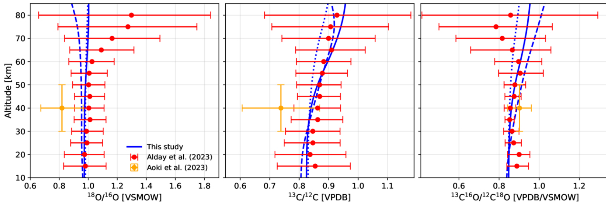
Figure 7. from Tatsuya Yoshida et al 2026 Planet. Sci. J. 7 doi:10.3847/PSJ/ae8762 https://dx.doi.org/10.3847/PSJ/ae8762 © 2026. The Author(s). Published by the American Astronomical Society.
