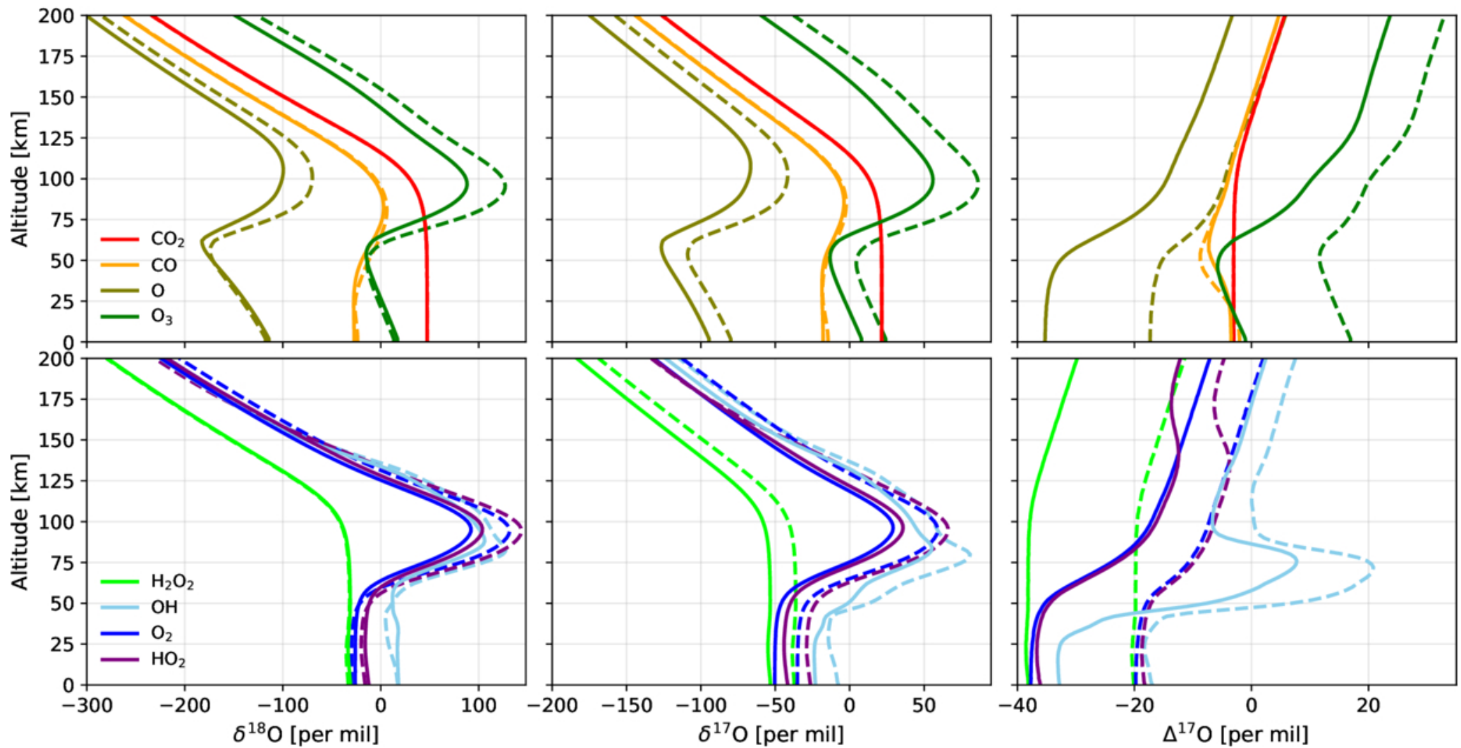
Figure 5. from Tatsuya Yoshida et al 2026 Planet. Sci. J. 7 doi:10.3847/PSJ/ae8762 https://dx.doi.org/10.3847/PSJ/ae8762 © 2026. The Author(s). Published by the American Astronomical Society.
