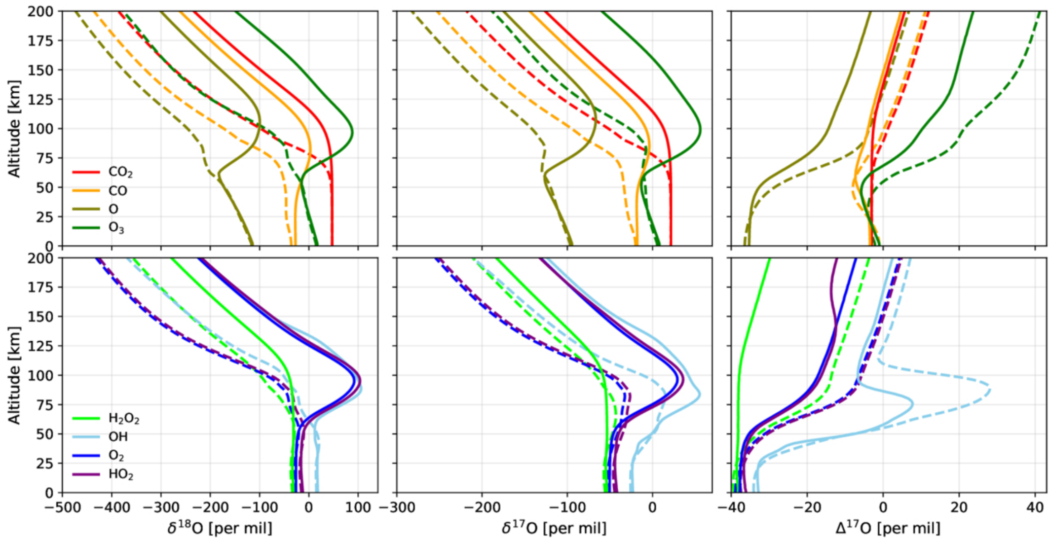
Figure 4. from Tatsuya Yoshida et al 2026 Planet. Sci. J. 7 doi:10.3847/PSJ/ae8762 https://dx.doi.org/10.3847/PSJ/ae8762 © 2026. The Author(s). Published by the American Astronomical Society.
