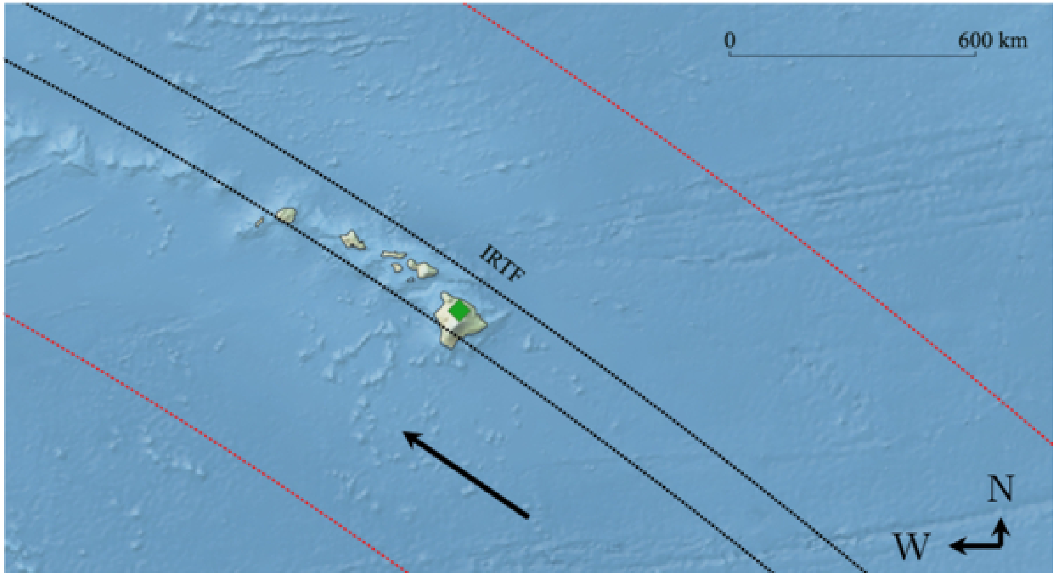
Figure 5. from Flavia L. Rommel et al 2026 Planet. Sci. J. 7 doi:10.3847/PSJ/ae84c6 https://dx.doi.org/10.3847/PSJ/ae84c6 © 2026. The Author(s). Published by the American Astronomical Society.
