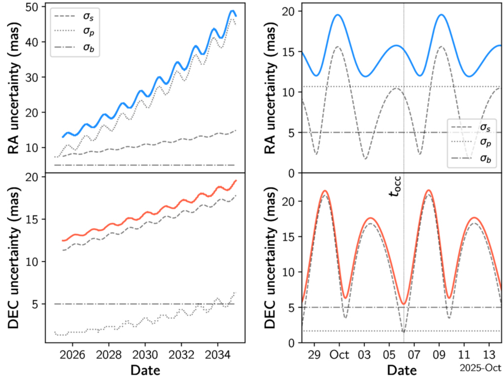
Figure 3. from Flavia L. Rommel et al 2026 Planet. Sci. J. 7 doi:10.3847/PSJ/ae84c6 https://dx.doi.org/10.3847/PSJ/ae84c6 © 2026. The Author(s). Published by the American Astronomical Society.
