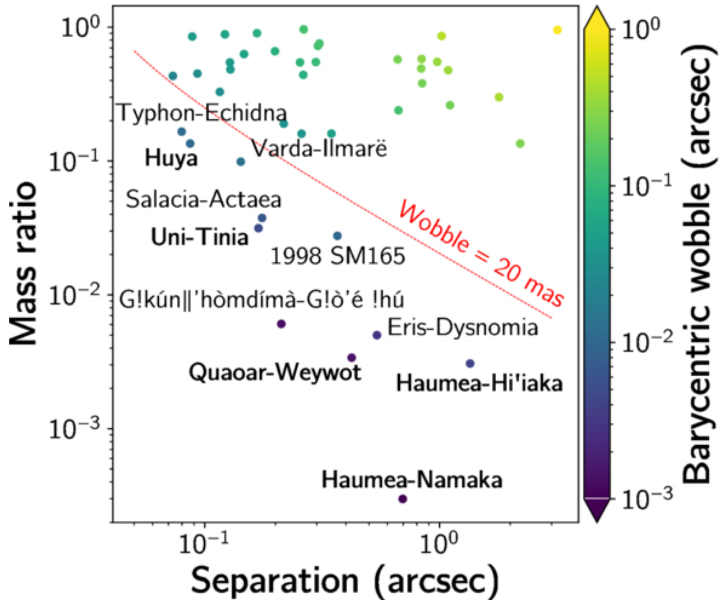
Figure 2. from Flavia L. Rommel et al 2026 Planet. Sci. J. 7 doi:10.3847/PSJ/ae84c6 https://dx.doi.org/10.3847/PSJ/ae84c6 © 2026. The Author(s). Published by the American Astronomical Society.
