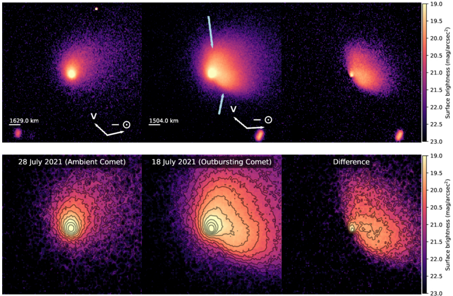
Figure 7. from Ky Huynh et al 2026 Planet. Sci. J. 7 doi:10.3847/PSJ/ae844f https://dx.doi.org/10.3847/PSJ/ae844f © 2026. The Author(s). Published by the American Astronomical Society.
