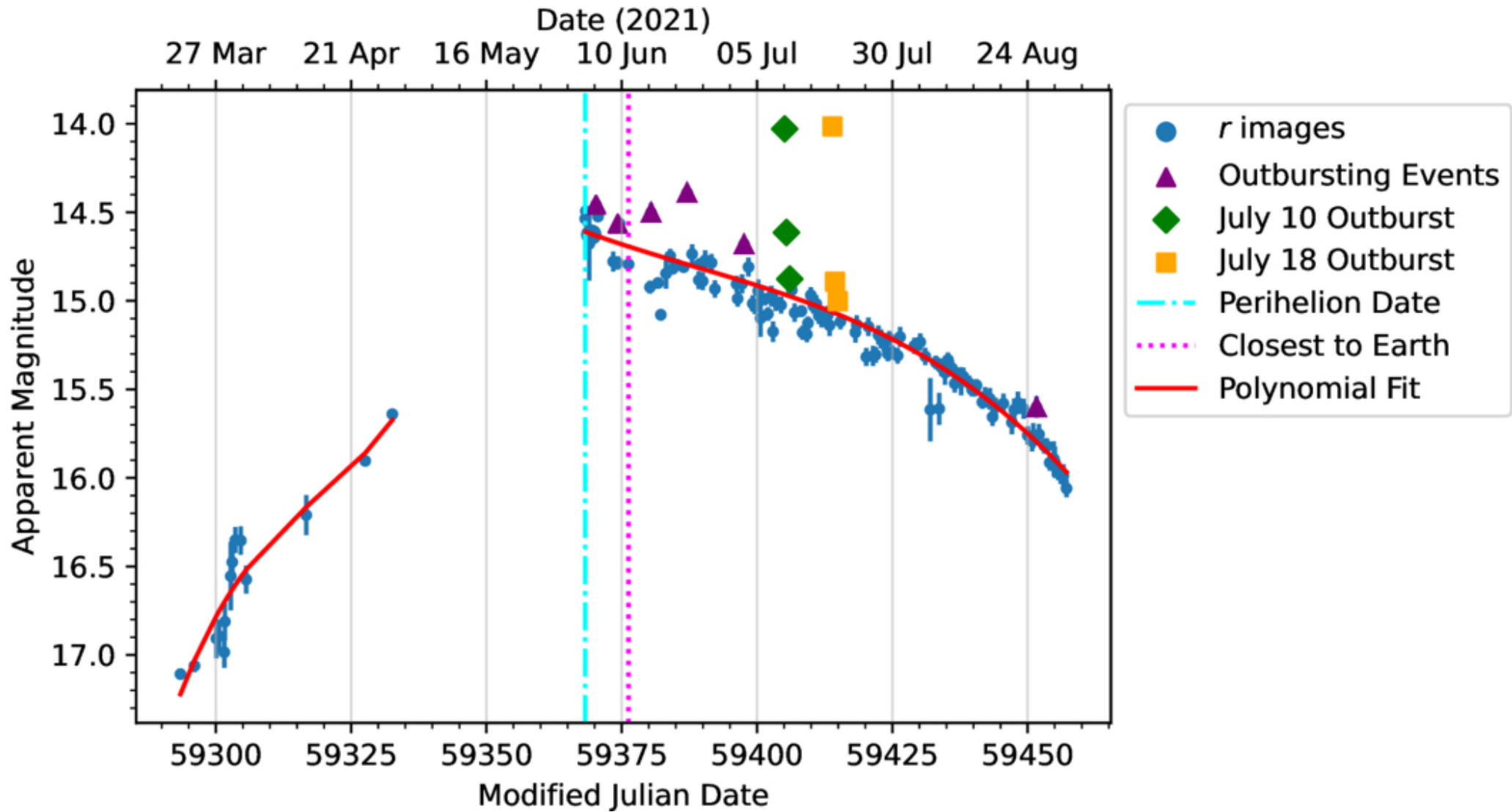
Figure 2. from Ky Huynh et al 2026 Planet. Sci. J. 7 doi:10.3847/PSJ/ae844f https://dx.doi.org/10.3847/PSJ/ae844f © 2026. The Author(s). Published by the American Astronomical Society.
