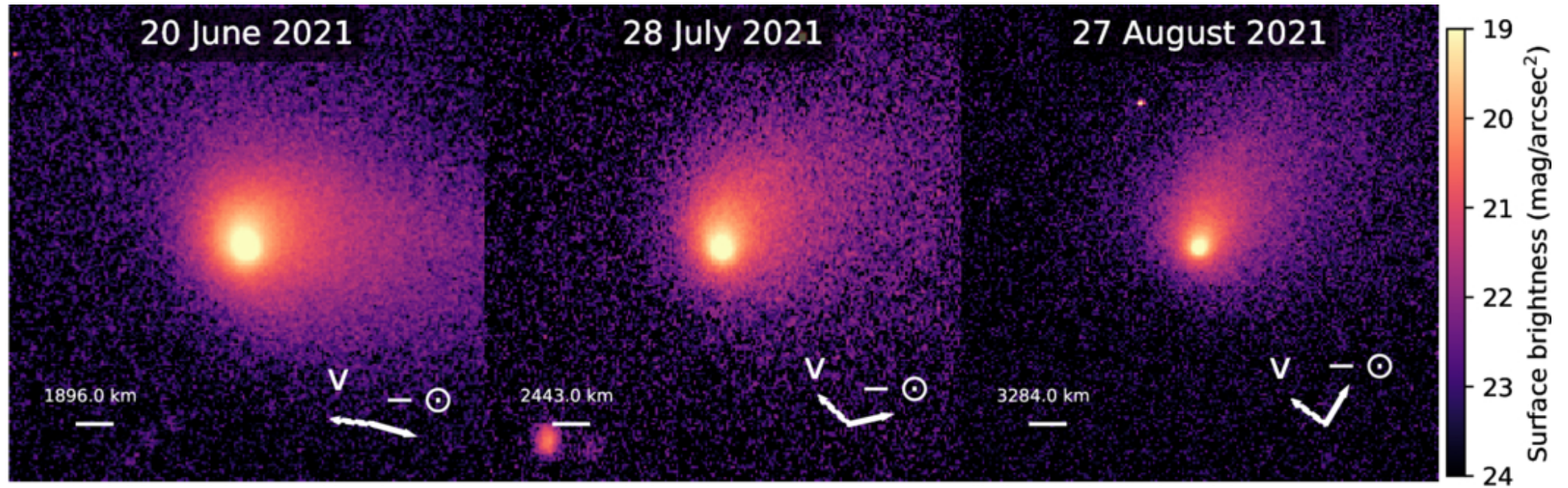
Figure 1. from Ky Huynh et al 2026 Planet. Sci. J. 7 doi:10.3847/PSJ/ae844f https://dx.doi.org/10.3847/PSJ/ae844f © 2026. The Author(s). Published by the American Astronomical Society.
