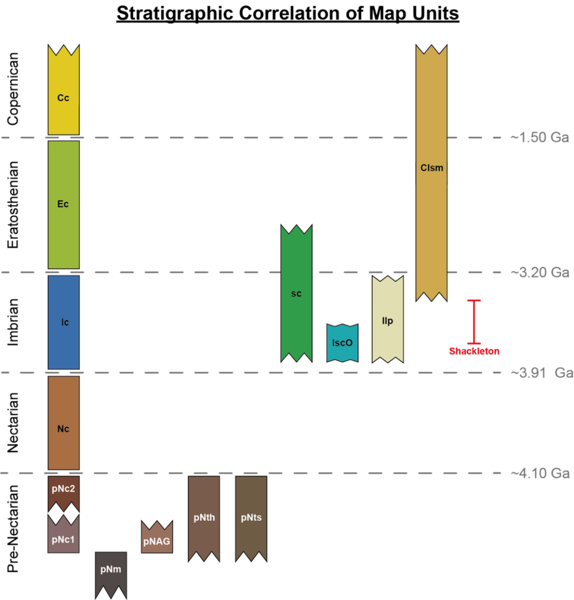
Figure 5. from Lukas Wueller et al 2026 Planet. Sci. J. 7 doi:10.3847/PSJ/ae8258 https://dx.doi.org/10.3847/PSJ/ae8258 © 2026. The Author(s). Published by the American Astronomical Society.
