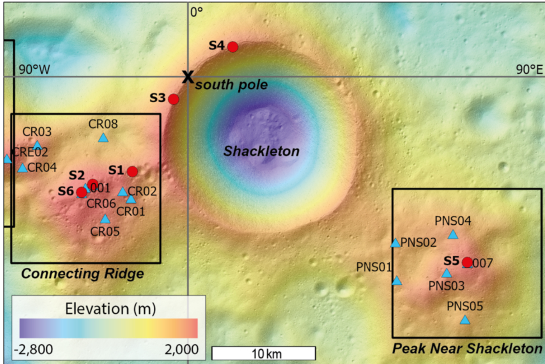
Figure 2. from Lukas Wueller et al 2026 Planet. Sci. J. 7 doi:10.3847/PSJ/ae8258 https://dx.doi.org/10.3847/PSJ/ae8258 © 2026. The Author(s). Published by the American Astronomical Society.
