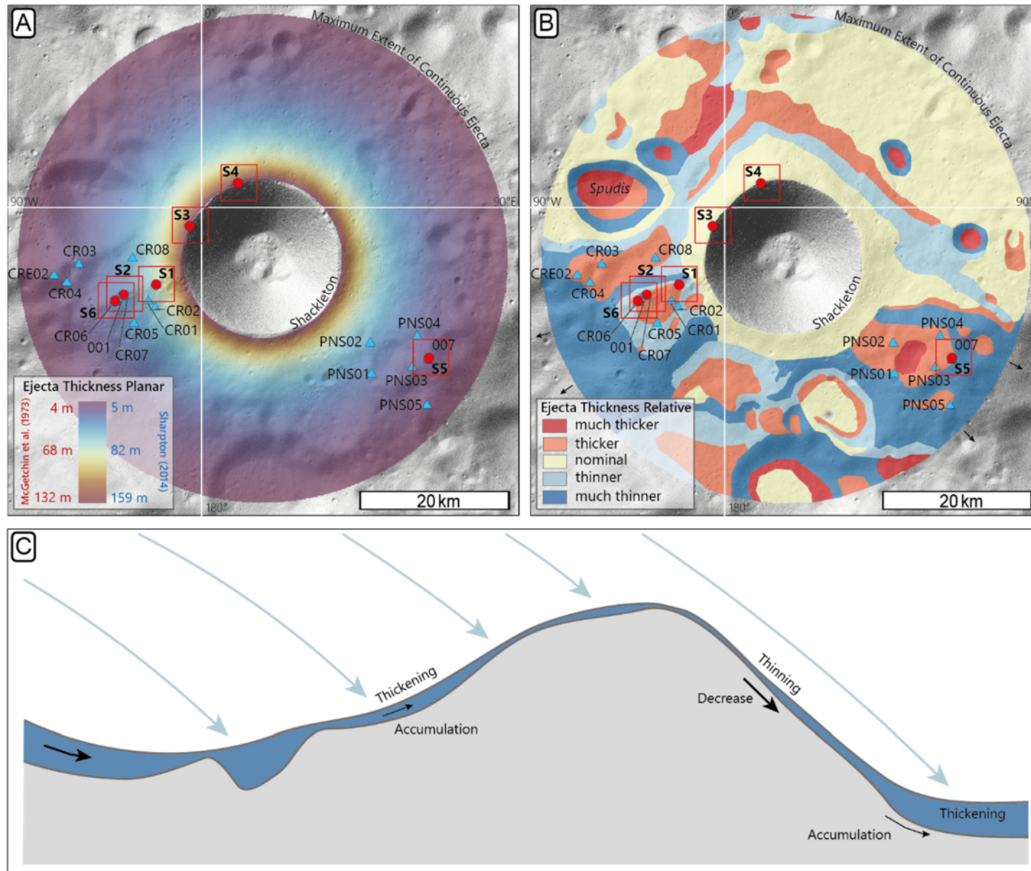
Figure 10. from Lukas Wueller et al 2026 Planet. Sci. J. 7 doi:10.3847/PSJ/ae8258 https://dx.doi.org/10.3847/PSJ/ae8258 © 2026. The Author(s). Published by the American Astronomical Society.
