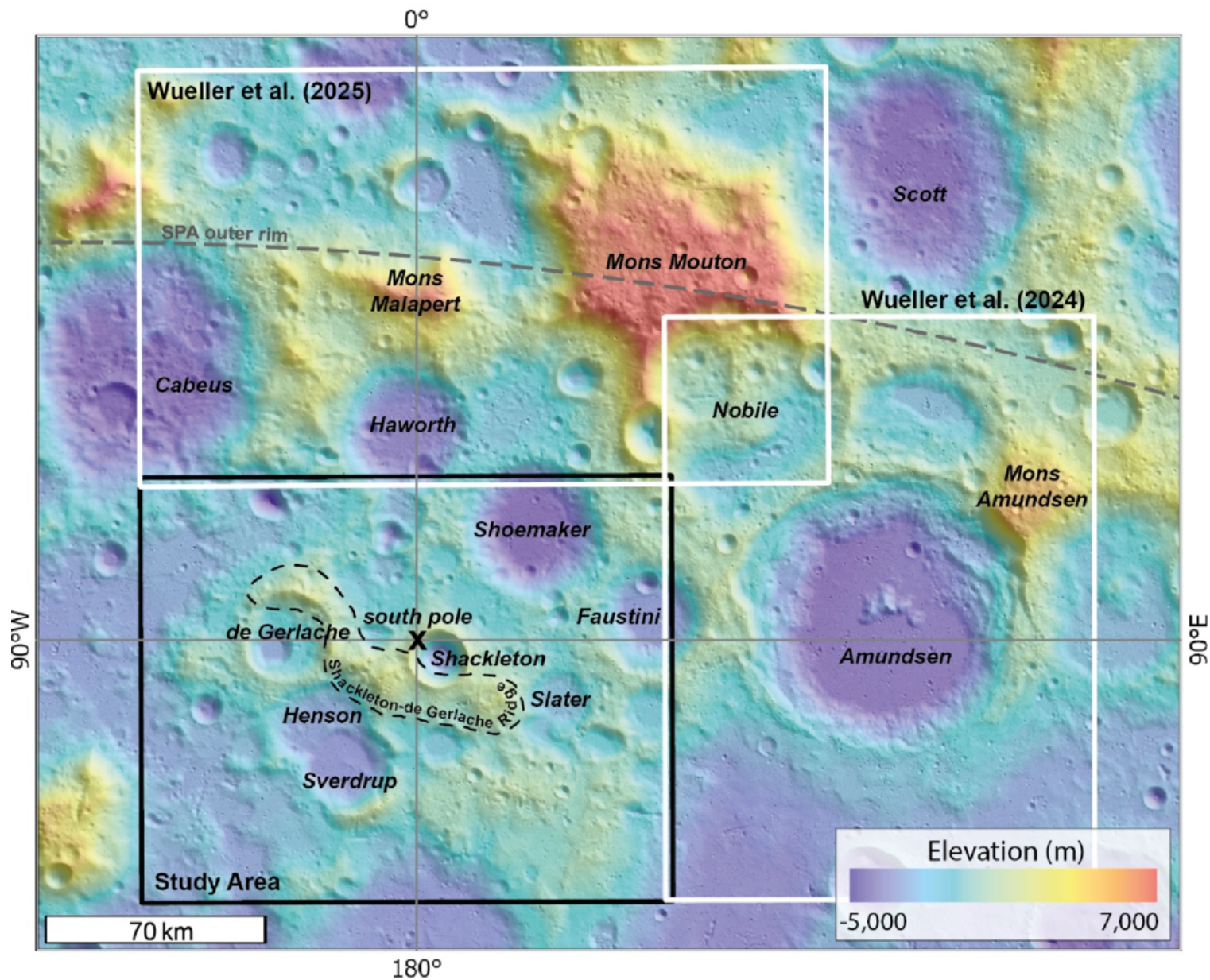
Figure 1. from Lukas Wueller et al 2026 Planet. Sci. J. 7 doi:10.3847/PSJ/ae8258 https://dx.doi.org/10.3847/PSJ/ae8258 © 2026. The Author(s). Published by the American Astronomical Society.
