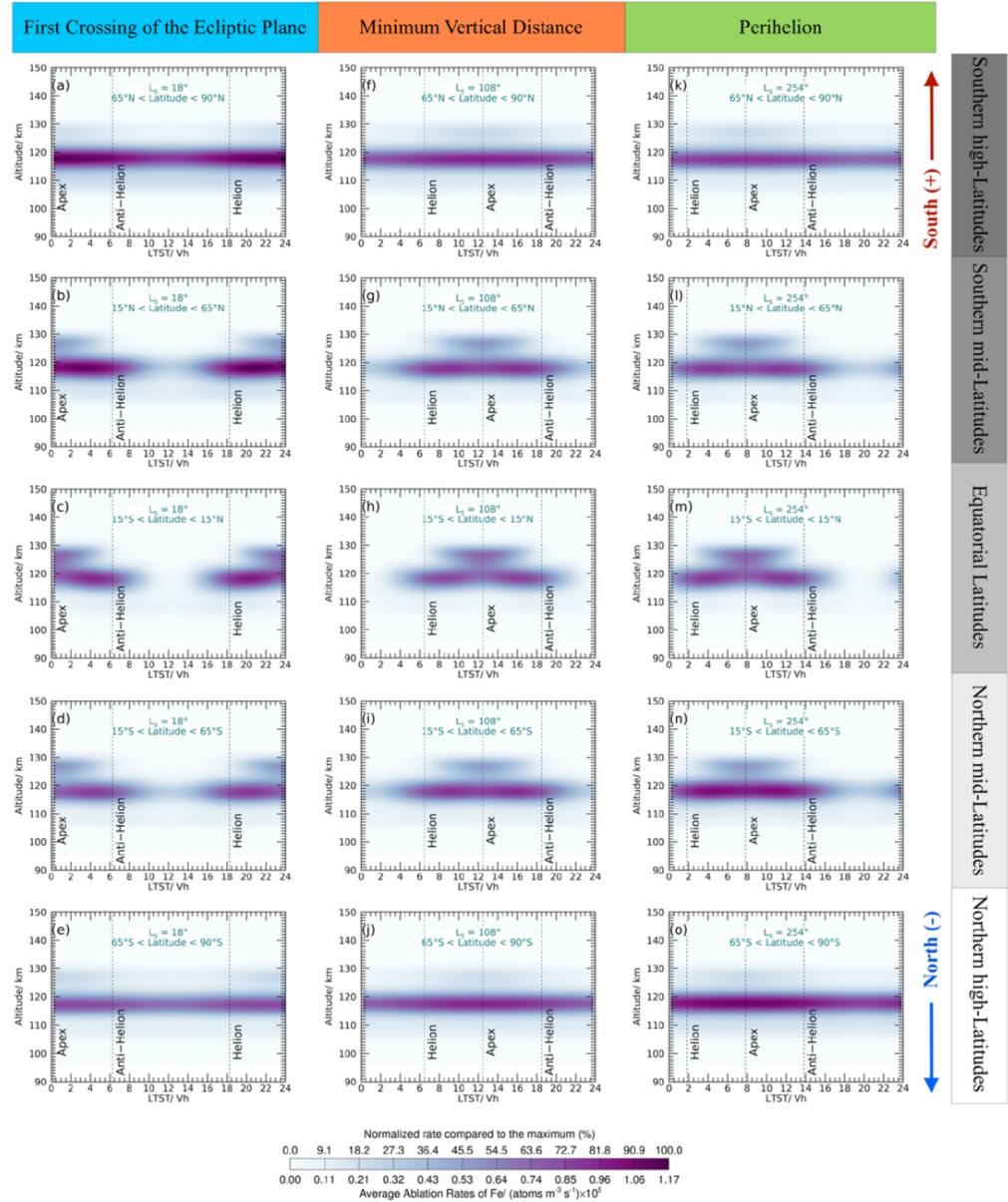
Figure 9. from Juan Diego Carrillo-Sánchez et al 2026 Planet. Sci. J. 7 doi:10.3847/PSJ/ae8257 https://dx.doi.org/10.3847/PSJ/ae8257 © 2026. The Author(s). Published by the American Astronomical Society.
