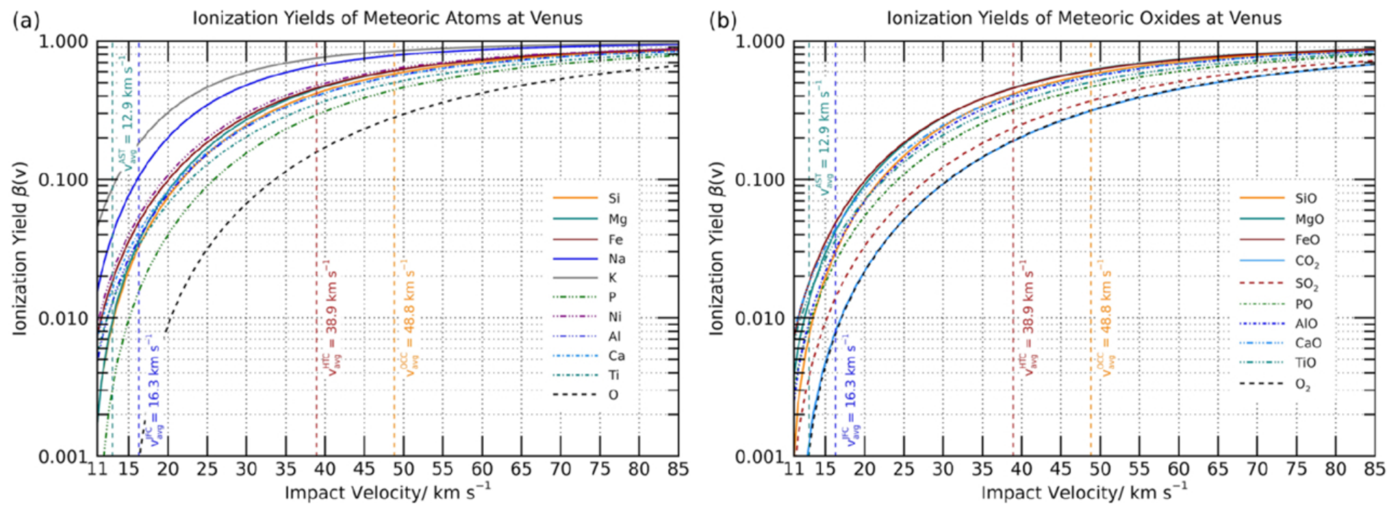
Figure 8. from Juan Diego Carrillo-Sánchez et al 2026 Planet. Sci. J. 7 doi:10.3847/PSJ/ae8257 https://dx.doi.org/10.3847/PSJ/ae8257 © 2026. The Author(s). Published by the American Astronomical Society.
