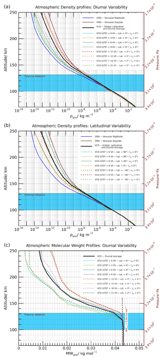
Figure 7. from Juan Diego Carrillo-Sánchez et al 2026 Planet. Sci. J. 7 doi:10.3847/PSJ/ae8257 https://dx.doi.org/10.3847/PSJ/ae8257 © 2026. The Author(s). Published by the American Astronomical Society.
